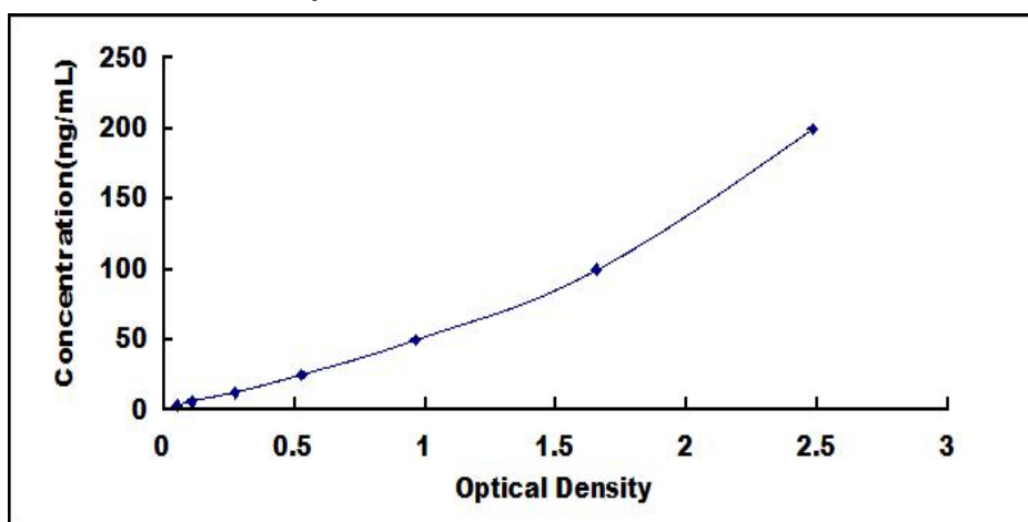
Typical Standard Curve for BGN ELISA.
