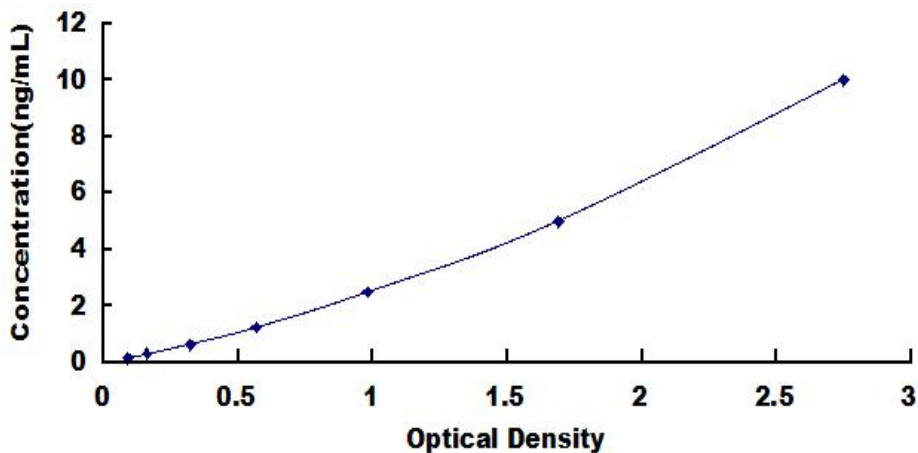
Typical Standard Curve for CaN ELISA.
