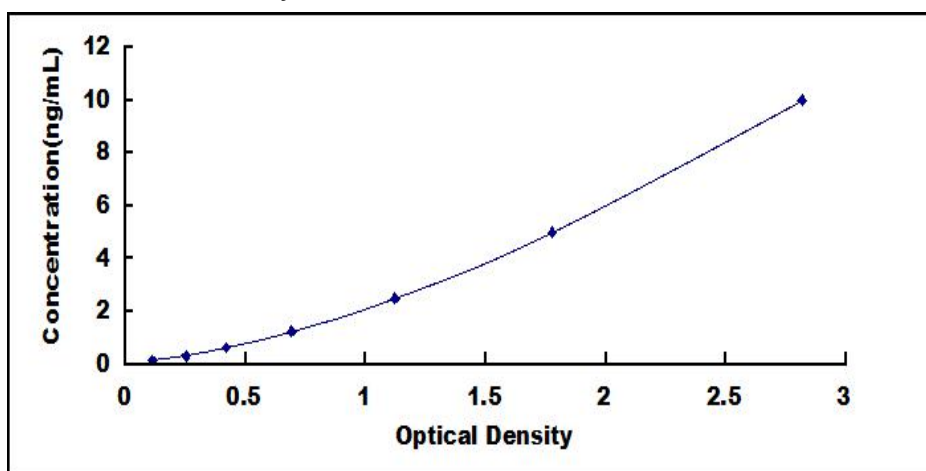
Typical Standard Curve for CASP5 ELISA.
