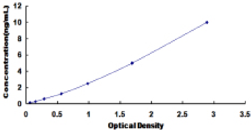
Typical Standard Curve for CAT2 ELISA.
