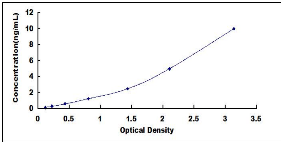
Typical Standard Curve for CDC42 ELISA.
