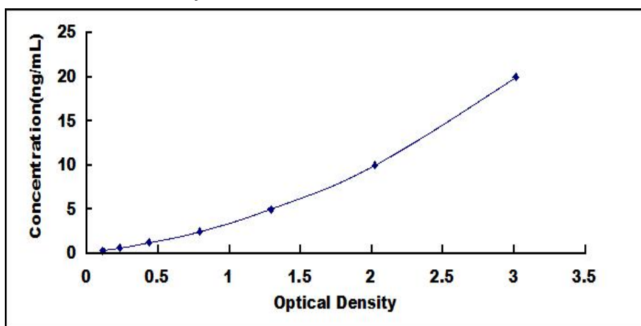
Typical Standard Curve for COL5a2 ELISA.
