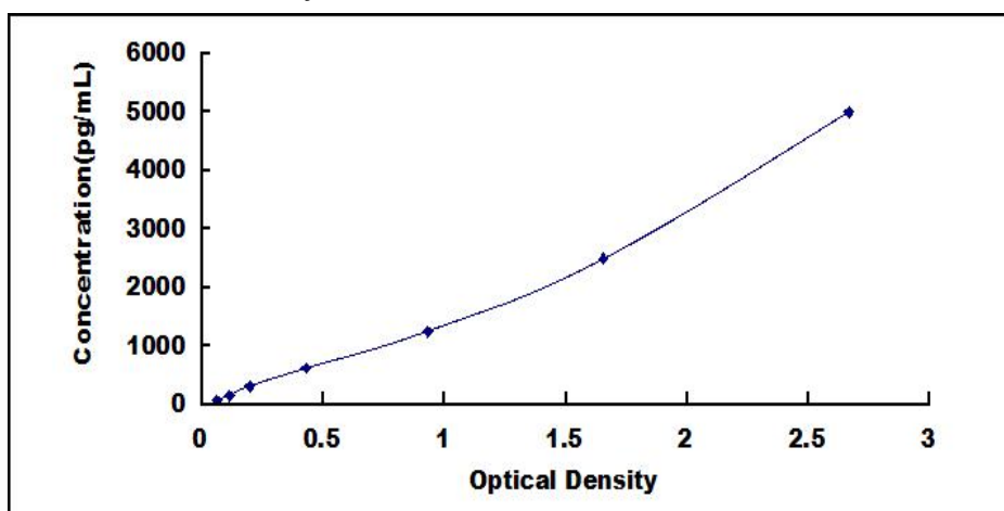
Typical Standard Curve for CD21 ELISA.
