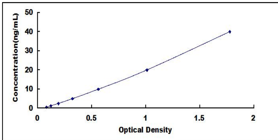
Typical Standard Curve for CRYaB ELISA.
