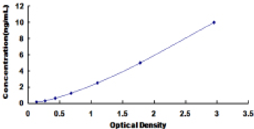
Typical Standard Curve for dLL4 ELISA.
