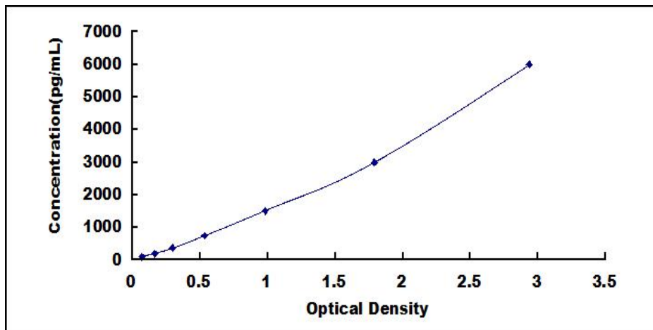
Typical Standard Curve for EGFL6 ELISA.
