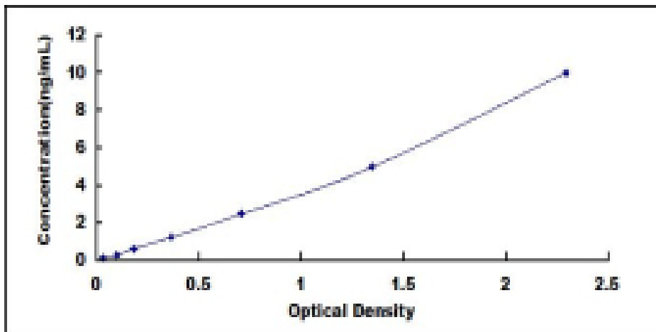
Typical Standard Curve for ERCC1 ELISA.
