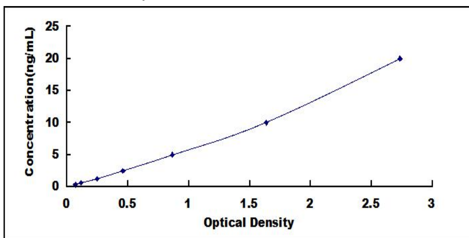
Typical Standard Curve for FcgBP ELISA.
