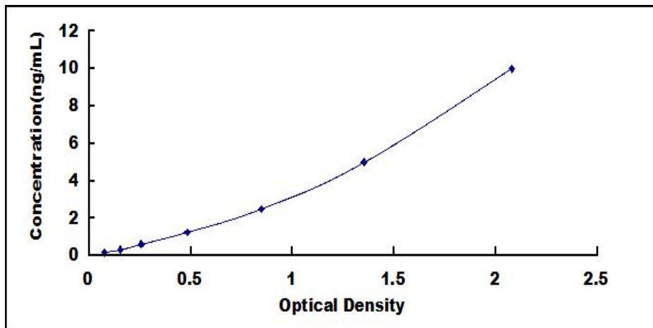
Typical Standard Curve for PYGL ELISA.
