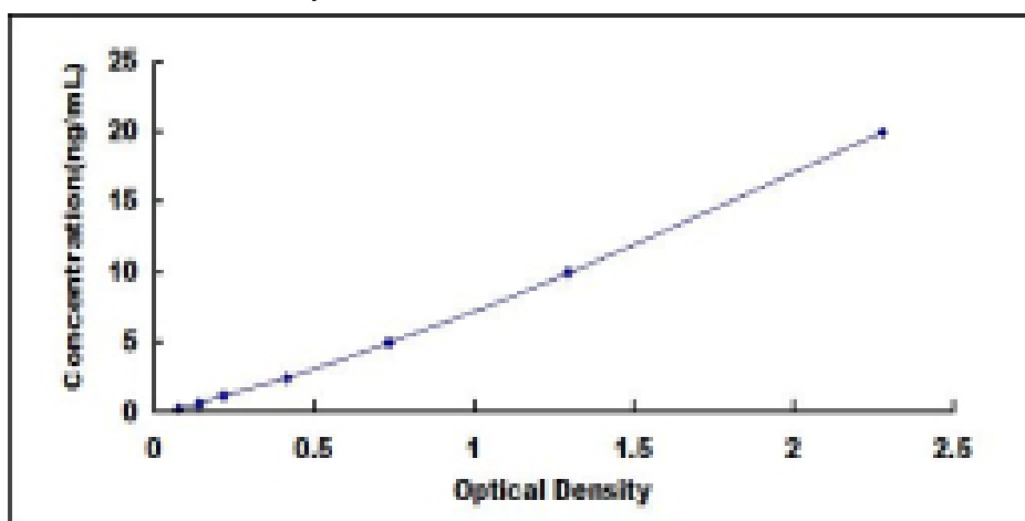
Typical Standard Curve for HADHb ELISA.
