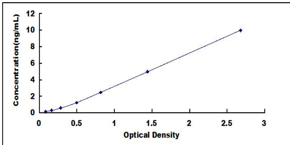
Typical Standard Curve for IPF ELISA.
