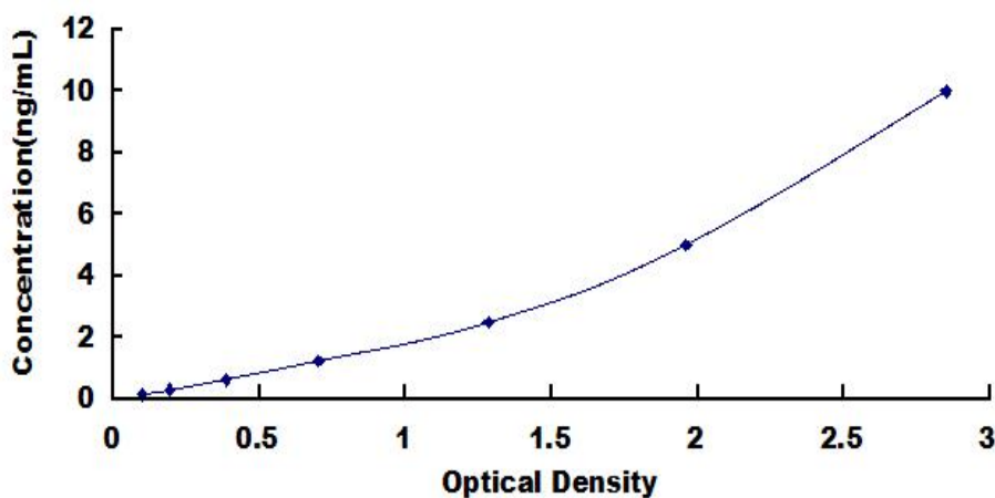
Typical Standard Curve for ITGb5 ELISA.
