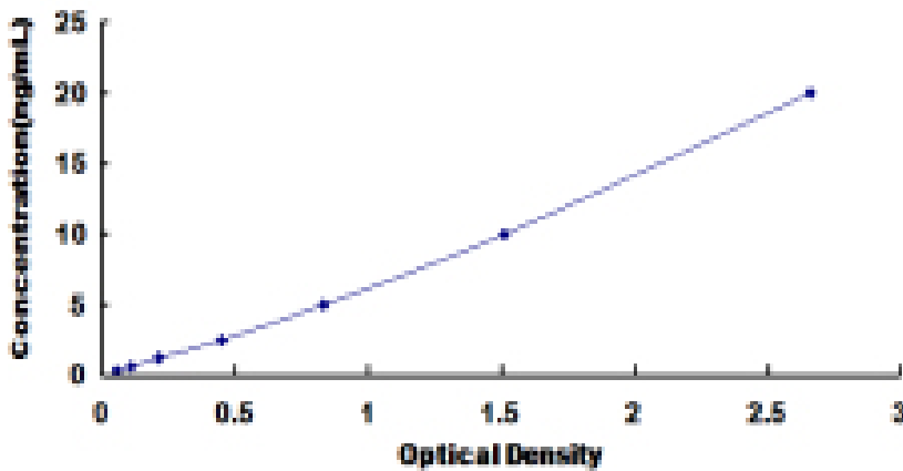
Typical Standard Curve for IQGAP1 ELISA.
