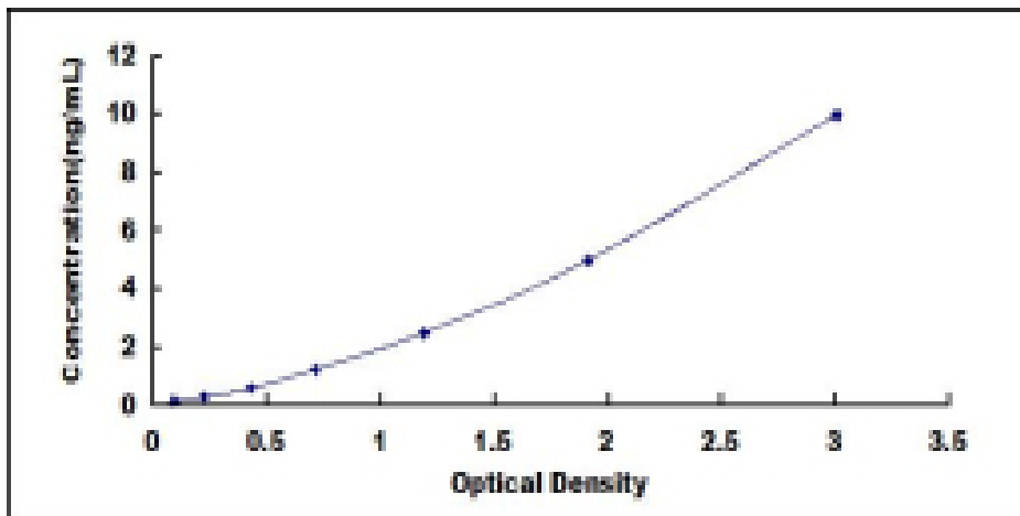
Typical Standard Curve for CK12 ELISA.
