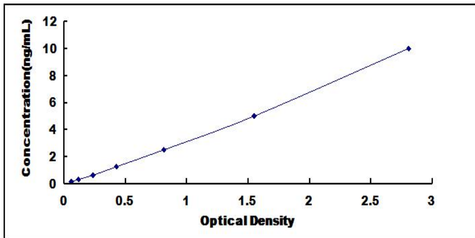
Typical Standard Curve for MST ELISA.
