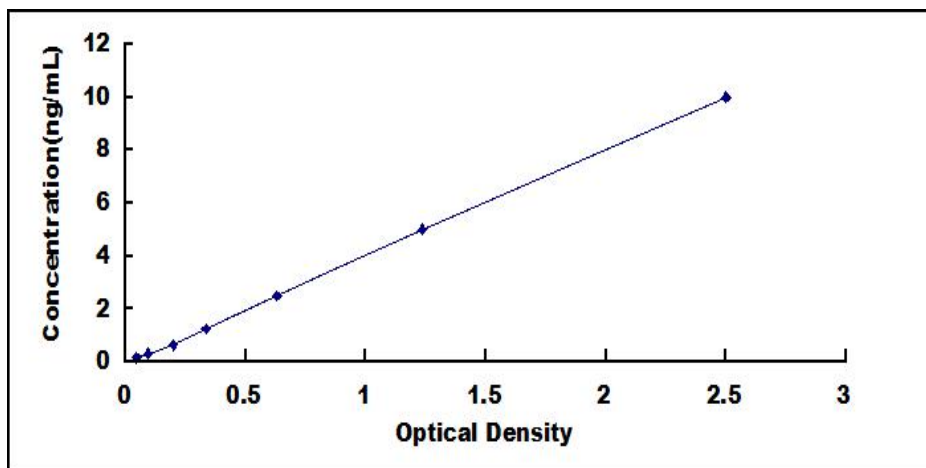
Typical Standard Curve for MSRA ELISA.
