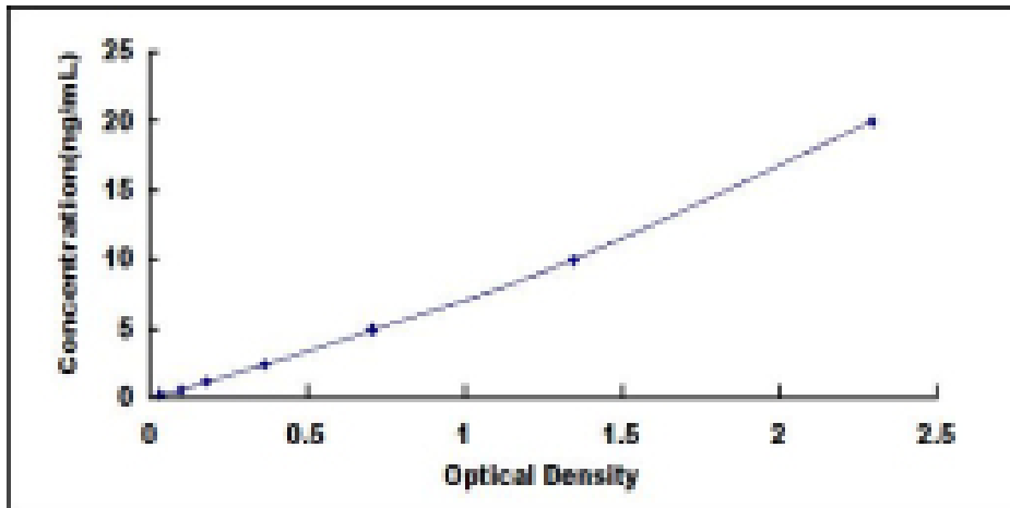
Typical Standard Curve for PAX9 ELISA.
