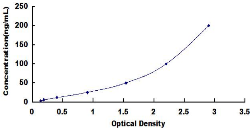
Typical Standard Curve for PON1 ELISA.
