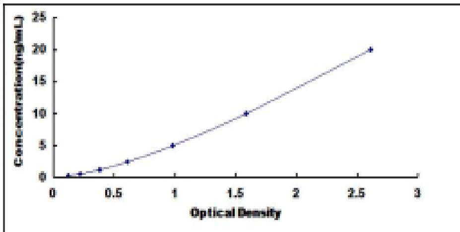
Typical Standard Curve for PTHR2 ELISA.
