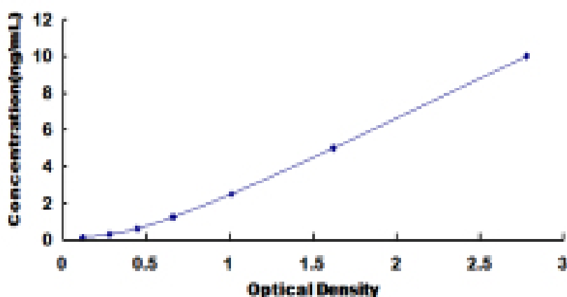
Typical Standard Curve for KCC4 ELISA.
