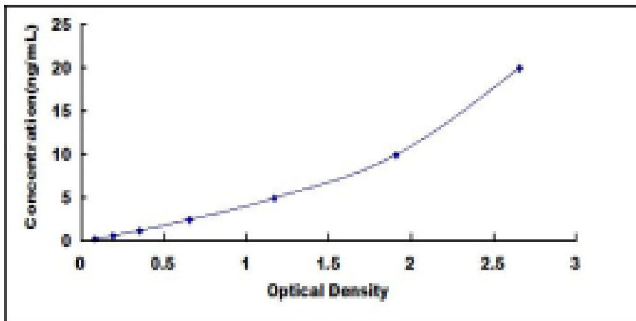
Typical Standard Curve for PGR ELISA.
