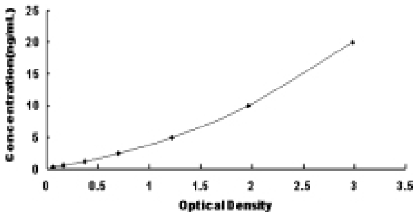
Typical Standard Curve for PRKAb1 ELISA.
