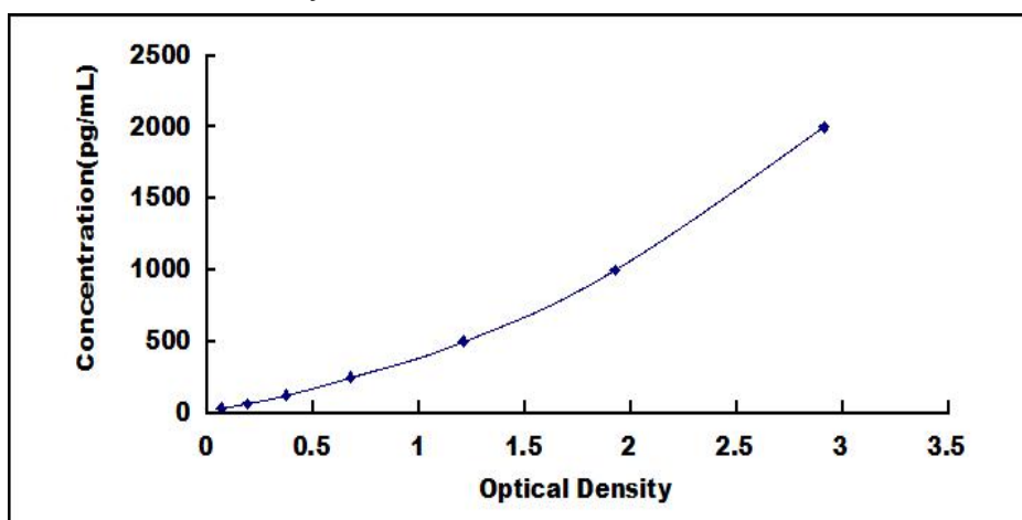
Typical Standard Curve for PCMT1 ELISA.
