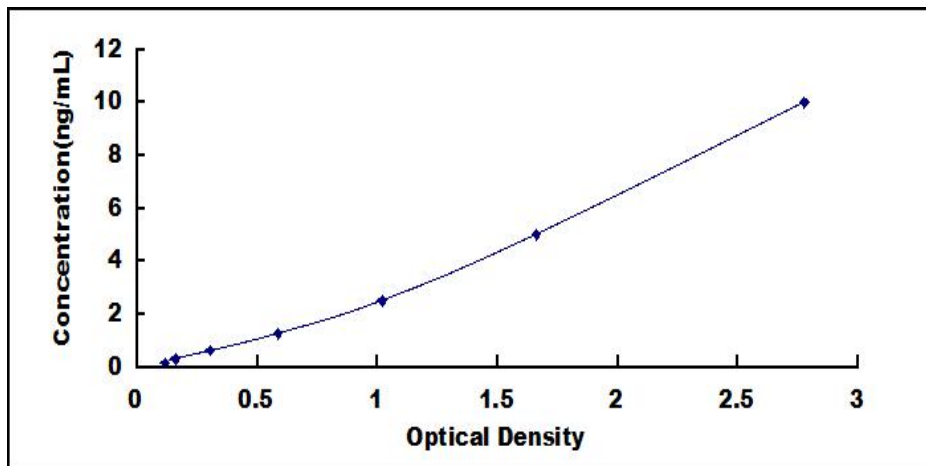
Typical Standard Curve for PROZ ELISA.
