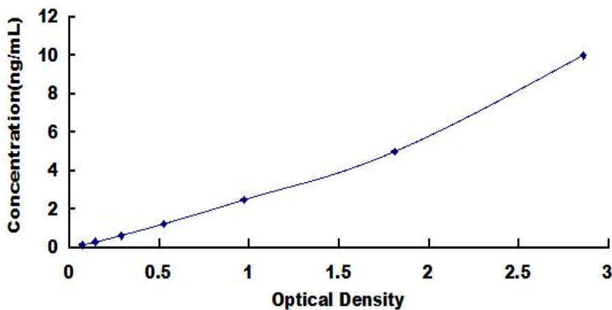
Typical Standard Curve for P2RY1 ELISA.
