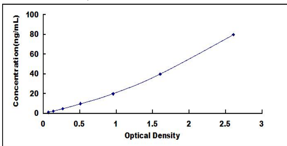
Typical Standard Curve for SCG2 ELISA.
