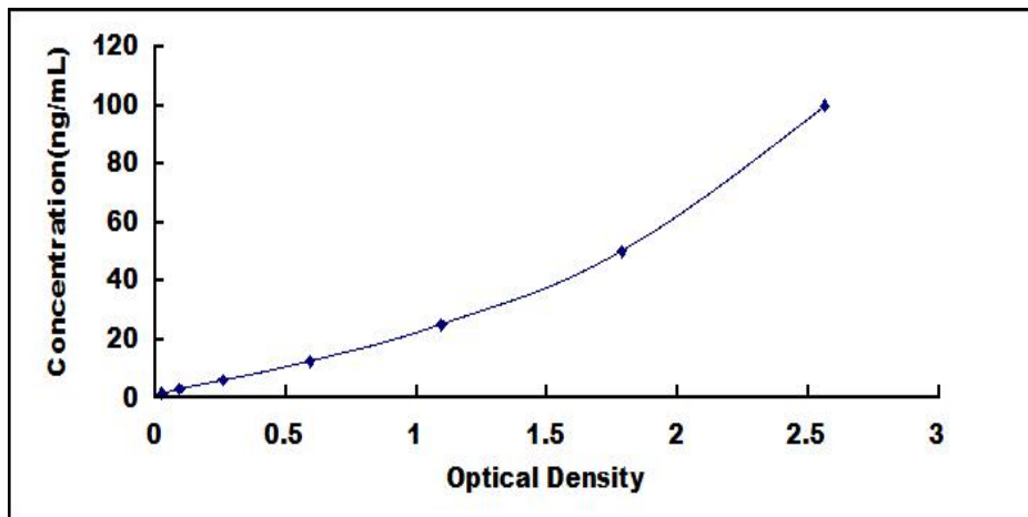
Typical Standard Curve for SAP ELISA.
