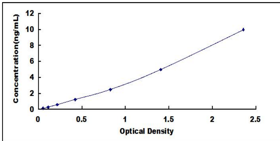
Typical Standard Curve for TAZ ELISA.
