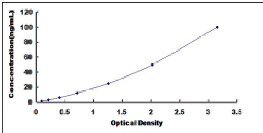
Typical Standard Curve for THOP1 ELISA.
