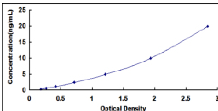
Typical Standard Curve for TDG ELISA.
