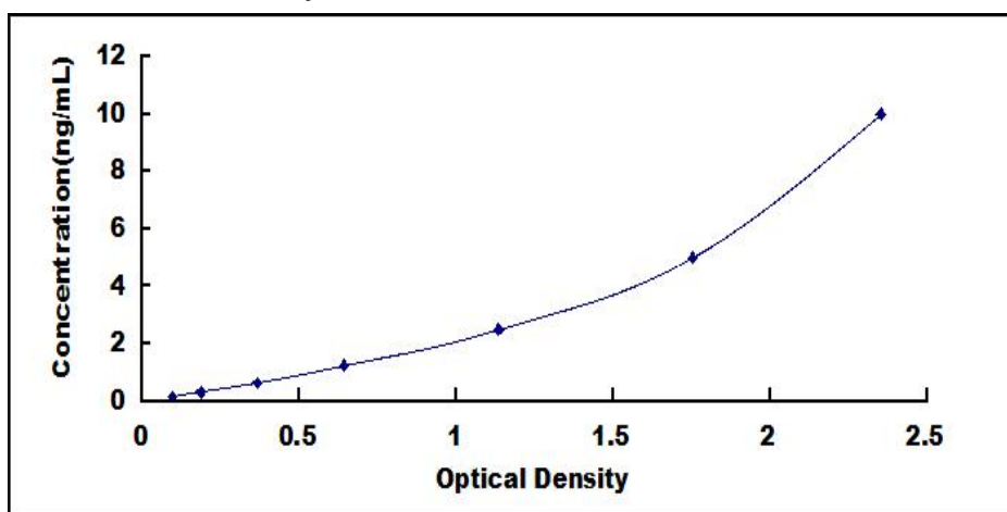
Typical Standard Curve for VNN1 ELISA.
