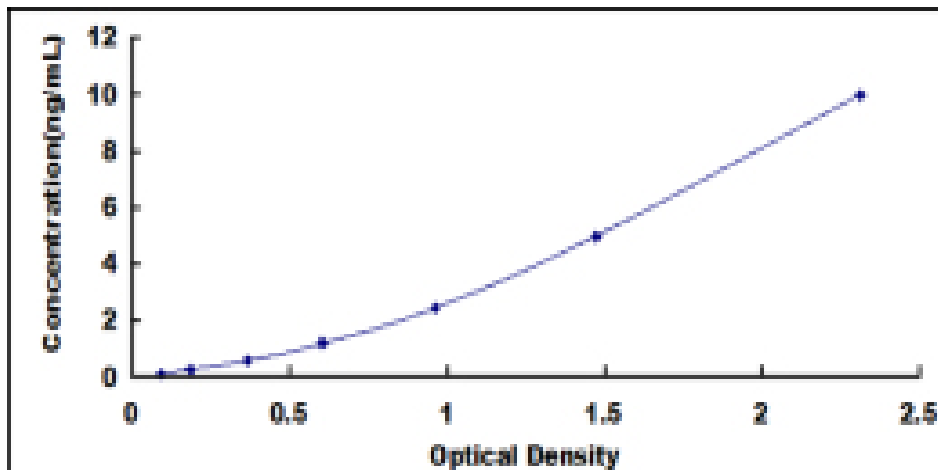
Typical Standard Curve for XPG ELISA.
