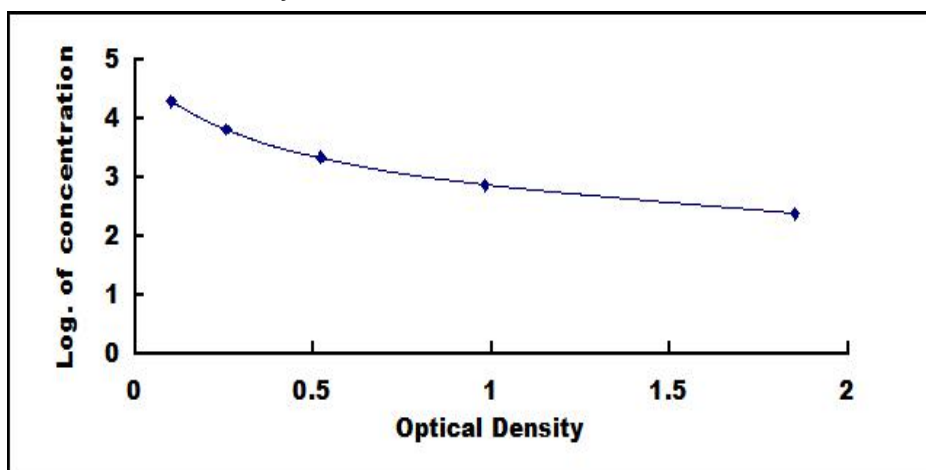
Typical Standard Curve for BSA ELISA.
