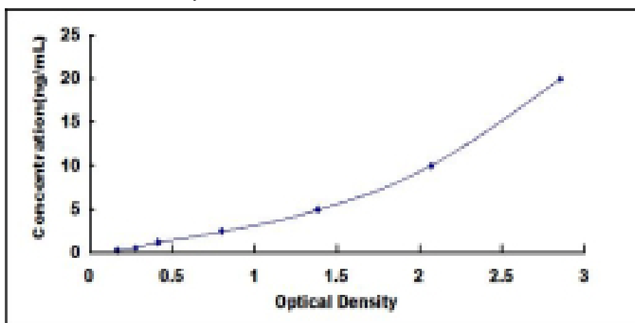
Typical Standard Curve for GJb6 ELISA.
