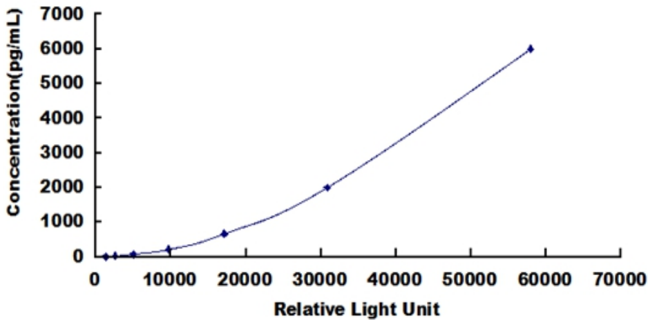
Typical Standard Curve for NGF ELISA.
