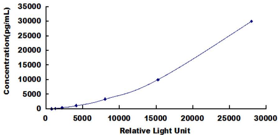
Typical Standard Curve for TIMP1 ELISA.
