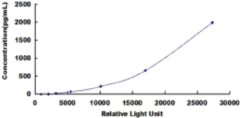
Typical Standard Curve for AIF ELISA.
