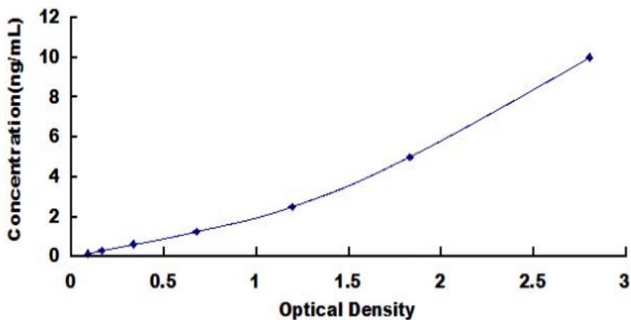
Typical Standard Curve for UPP1 ELISA.
