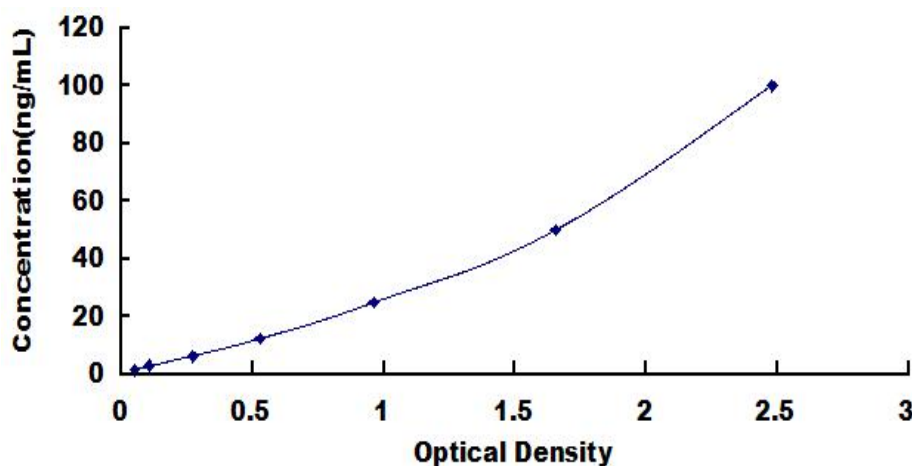
Typical Standard Curve for HMGCRC ELISA.
