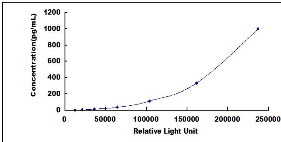
Typical Standard Curve for IFNa13 ELISA.
