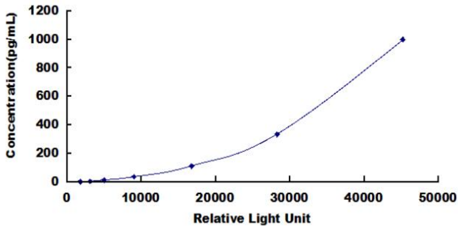
Typical Standard Curve for IL35 ELISA.
