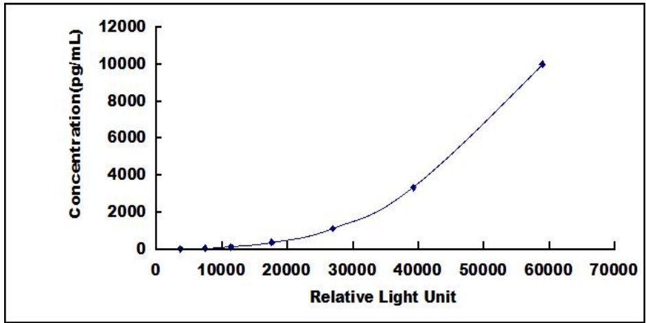
Typical Standard Curve for UBE2L3 ELISA.
