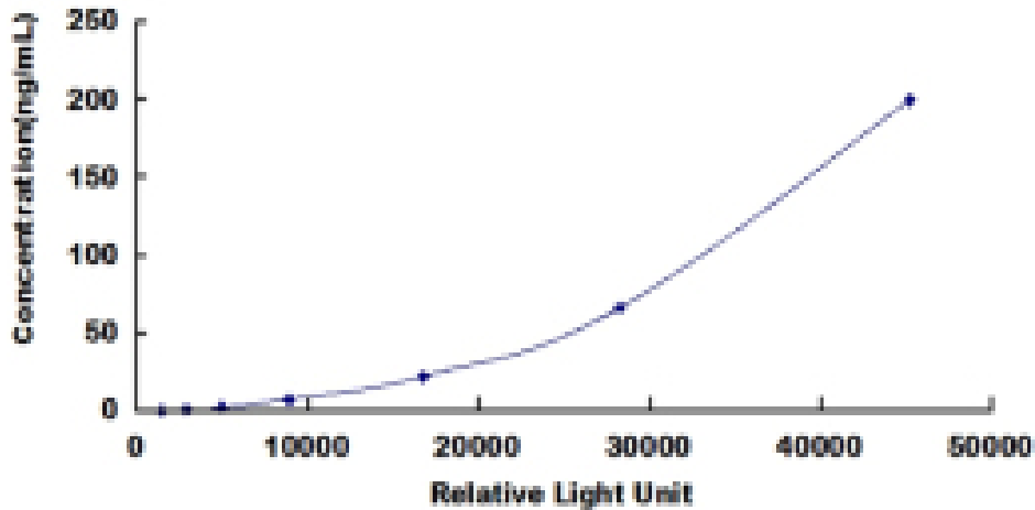
Typical Standard Curve for C4c ELISA.
