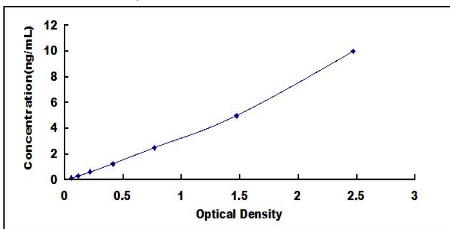
Typical Standard Curve for TCF7L2 ELISA.
