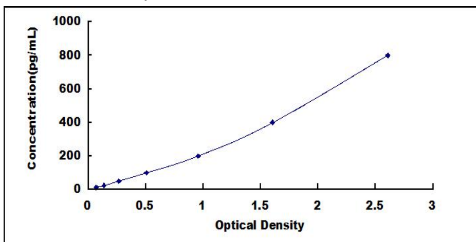
Typical Standard Curve for C5b-9 ELISA.
