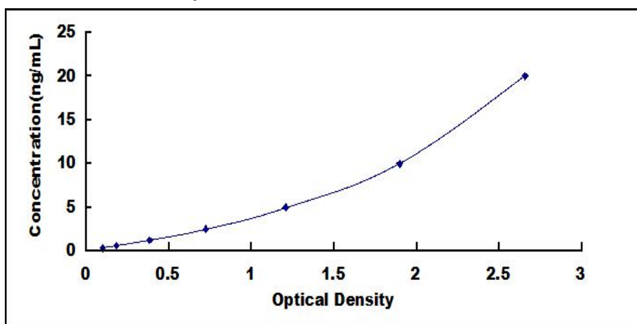
Typical Standard Curve for BPGM ELISA.
